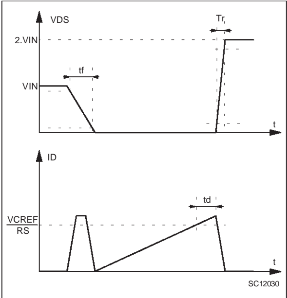
Figure 1: Switching Times
