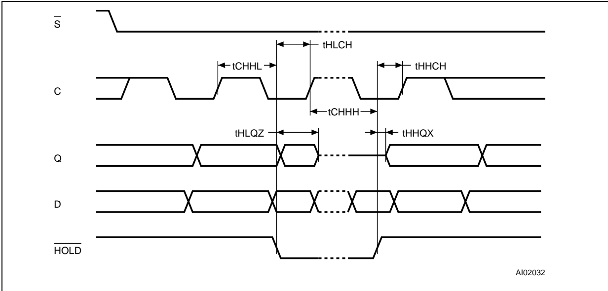
Figure 15. Hold Timing
