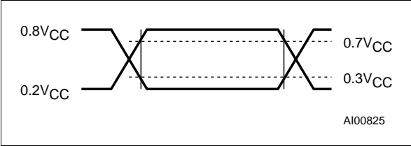
Figure 13. AC Testing Input Output Waveforms
