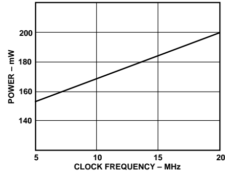
Figure 13. Typical Power Dissipation vs. Clock Frequency to +5 V all digital inputs readily interface with 5 V CMOS logic.
