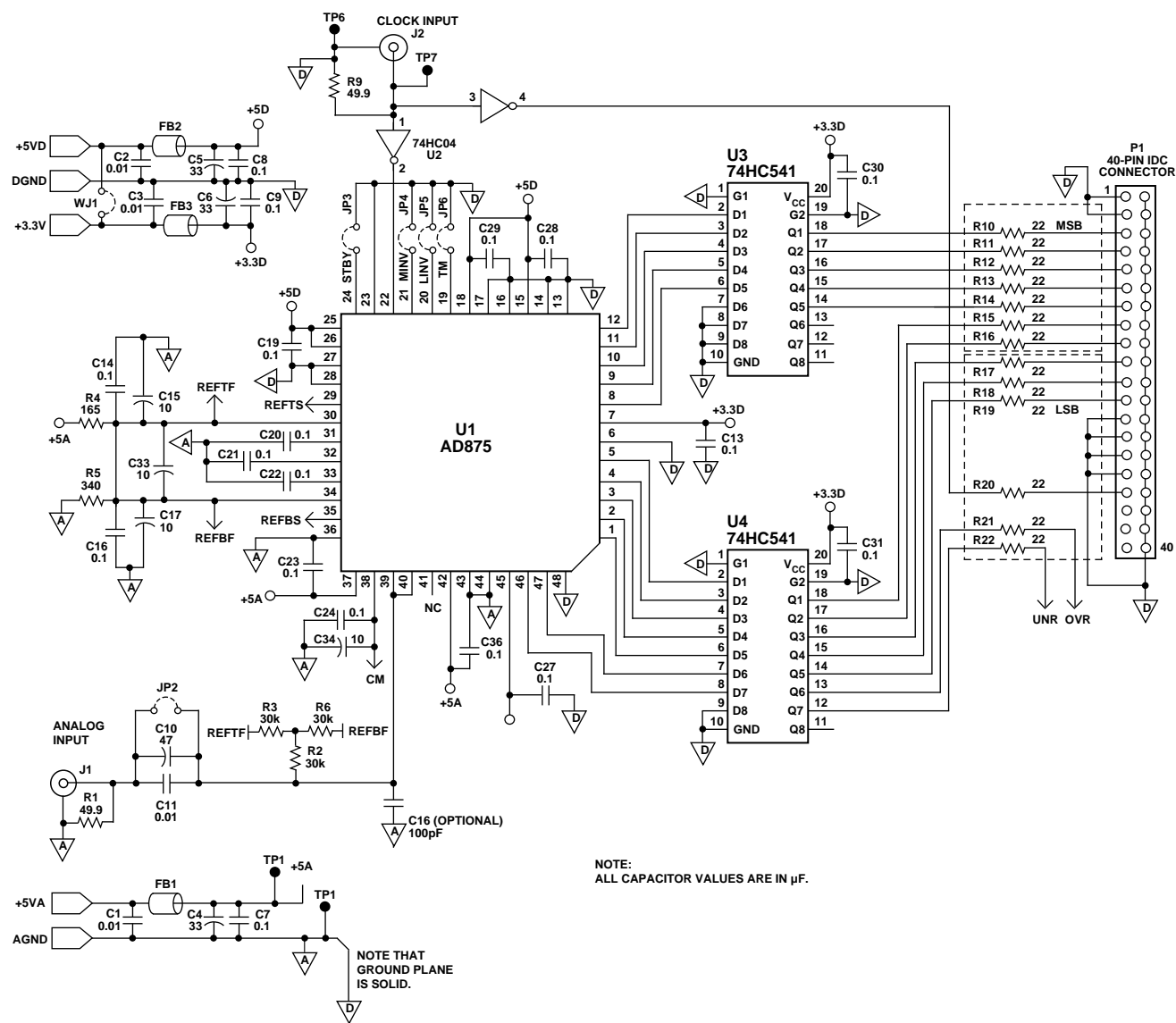
Figure 20. AD875 Evaluation Board Schematic
