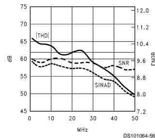
Dynamics at 30 MSPS
