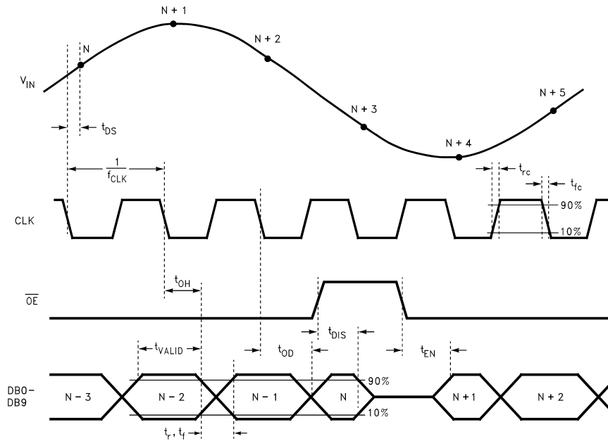
FIGURE 1. ADC10030 Timing Diagram
