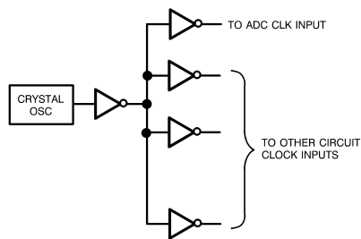
FIGURE 8. Isolating the ADC Clock from Digital Circuitry
