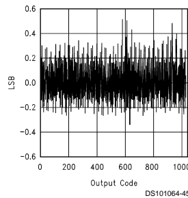
Typical DNL
