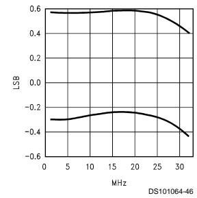
DNL vs f_{CLK}
