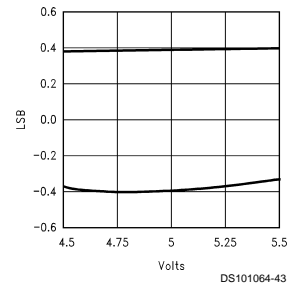
INL vs V_A
