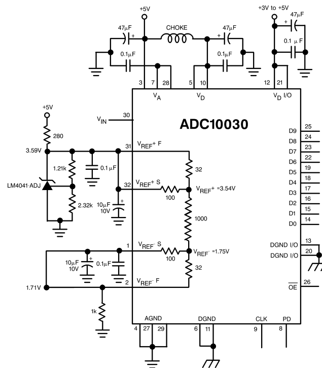
FIGURE 5. Improved Low Component Count Reference Biasing
