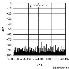
Spectral Response at 30 MSPS
