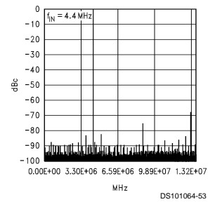
Spectral Response at 27 MSPS
