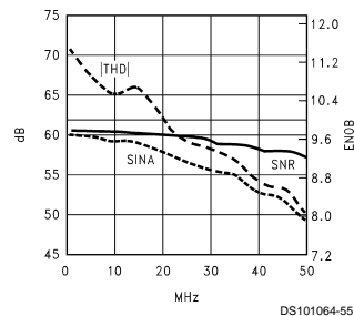
Dynamics at 27 MSPS
