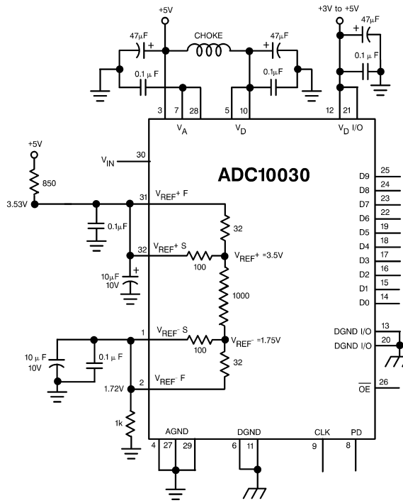
FIGURE 4. Simple, Low Component Count Reference Biasing
