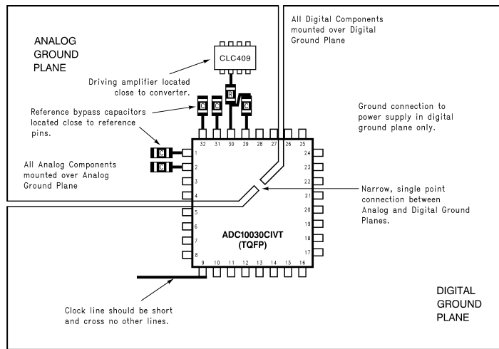
FIGURE 7. An Acceptable Layout Pattern for the ADC10030
