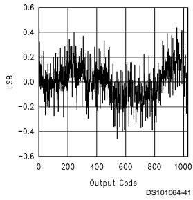
Typical INL
