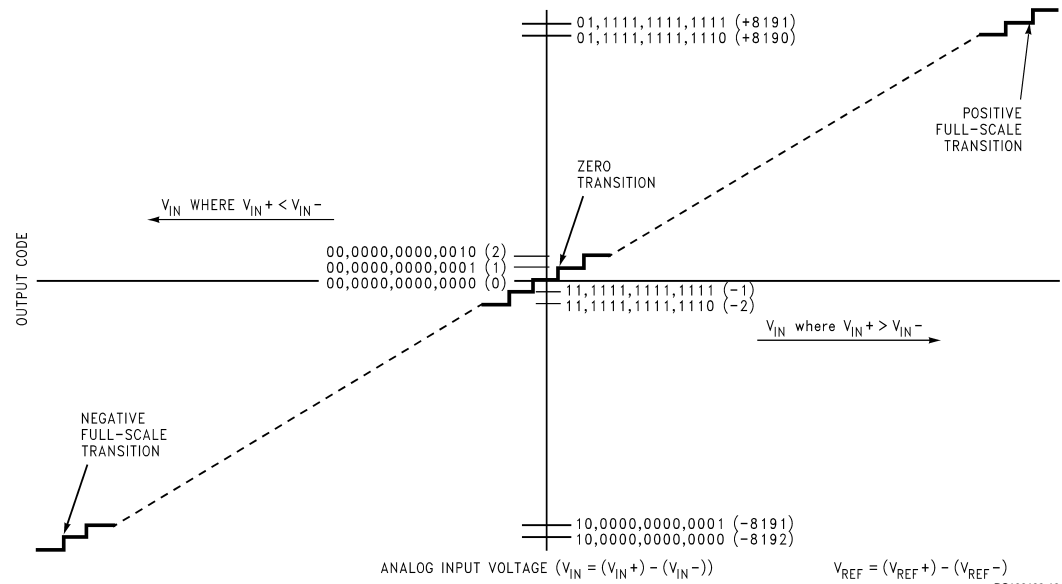
FIGURE 1. Transfer Characteristics
