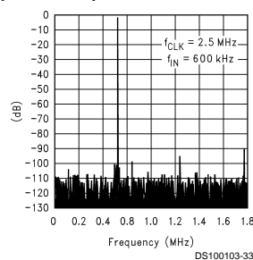
Spectral Response
