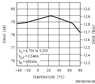
SINAD & ENOB vs Temperature
