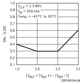
DNL vs V_{REF} and Temperature
