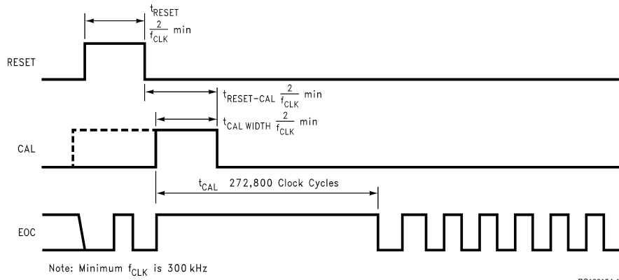
TIMING DIAGRAM 2. Reset and Calibration
