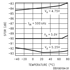
SFDR vs Temperature and f_{IN}
