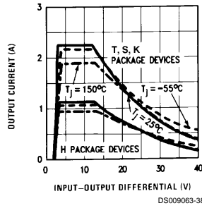
Current Limit
