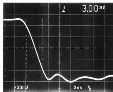
FIGURE 18. LM1208 Fall Time
