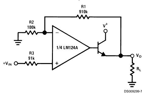
Power Amplifier
