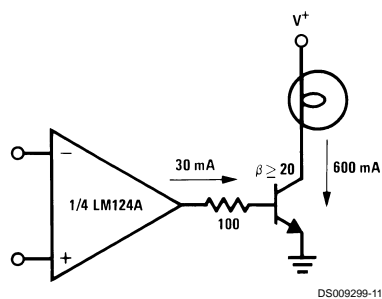
Lamp Driver
