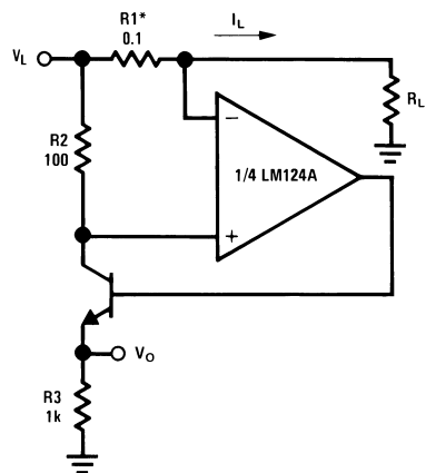
Current Monitor
