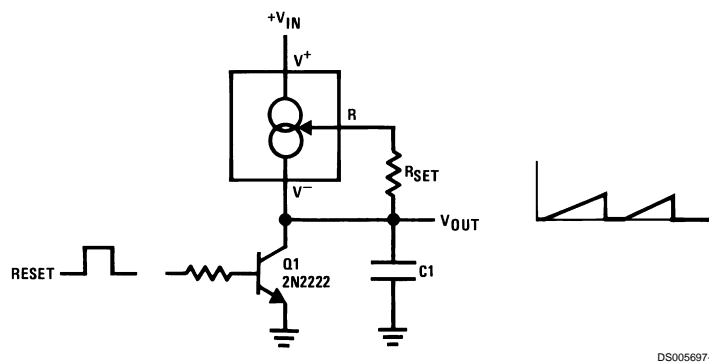
Ramp Generator
