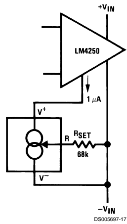
Micropower Bias
