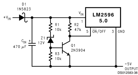
FIGURE 23. Undervoltage Lockout for Inverting Regulator
