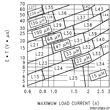
FIGURE 7. LM2596-ADJ
