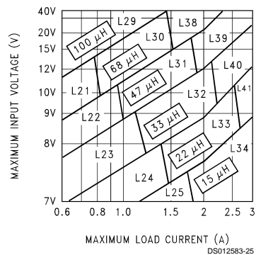
FIGURE 5. LM2596-5.0
