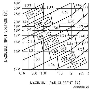
FIGURE 6. LM2596-12
