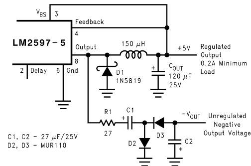
FIGURE 33. Charge Pump for Generating a Low Current, Negative Output Voltage
