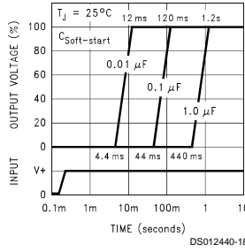
Soft-start Response
