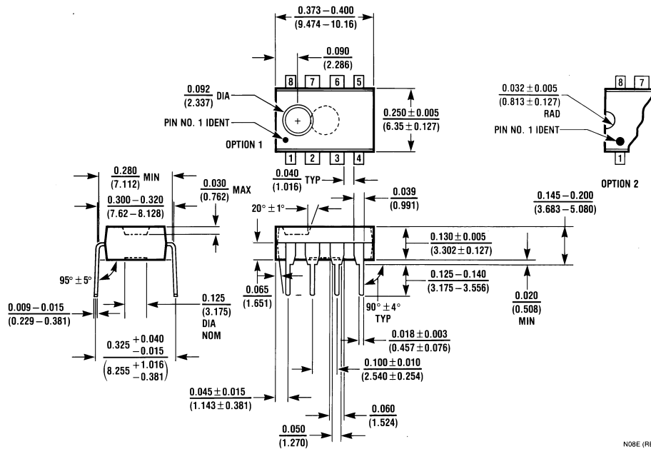
8-Lead (0.300" Wide) Molded Dual-In-Line Package, Order Number LM2597N-3.3, LM2597N-5.0, LM2597N-12 or LM2597N-ADJ LM2597HVN-3.3, LM2597HVN-5.0, LM2597HVN-12 or LM2597HVN-ADJ NS Package Number N08E
