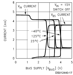
V_{IN} and V_{BS} Current vs V_{BS} and Temperature
