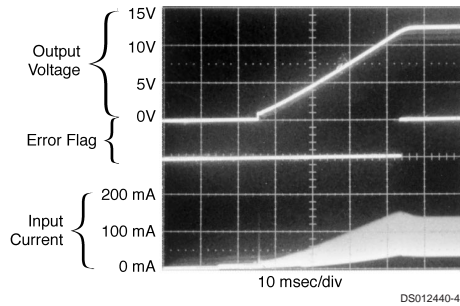
FIGURE 25. Output Voltage, Input Current, Error Flag Signal, at Start-Up, WITH Soft-start
