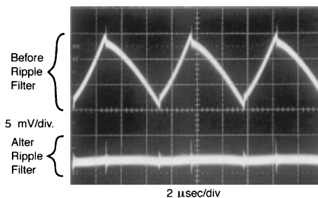
FIGURE 19. Post Ripple Filter Waveform
