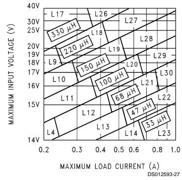
FIGURE 6. LM2598-12
