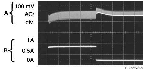
A: Output Voltage, 100 mV/div. (AC) B: 250 mA to 750 mA Load Pulse
