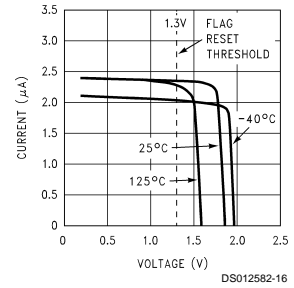
Daisy Pin Current
