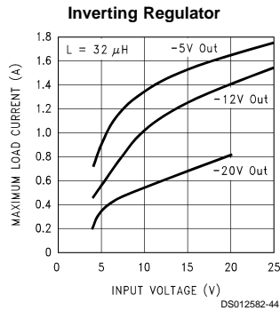
FIGURE 27. Maximum Load Current for Inverting Regulator Circuit
