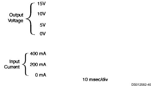
FIGURE 23. Output Voltage, Input Current, at Start-Up, WITH Soft-start
