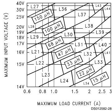
FIGURE 6. LM2599-12
