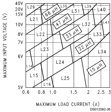
FIGURE 4. LM2599-3.3
