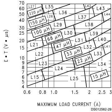
FIGURE 7. LM2599-ADJ
