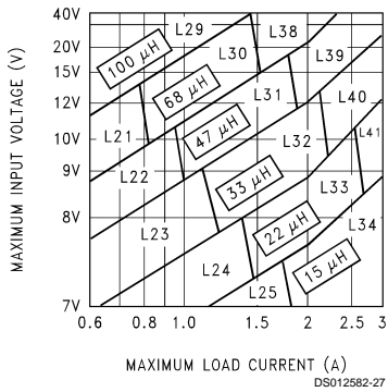
FIGURE 5. LM2599-5.0
