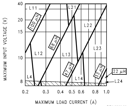
FIGURE 4. LM2675-3.3
