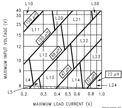
FIGURE 5. LM2675-5.0
