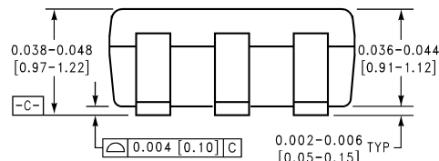
6-Lead Small Outline Package (M6) NS Package Number MA06A
