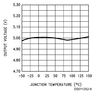
Output Voltage
