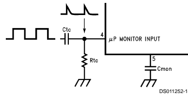
FIGURE 2. Monitoring Square Wave \mu\text{P} Signals
