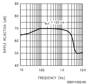
Ripple Rejection ( V_{BUF} )
