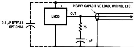
FIGURE 4. LM35 with R-C Damper
