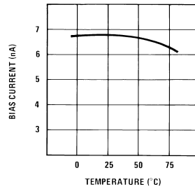
Operating Input Bias Current vs Temperature
