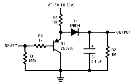
FIGURE 1. Half-Wave Peak Detector
