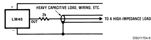
FIGURE 4. LM45 with Decoupling from Capacitive Load
