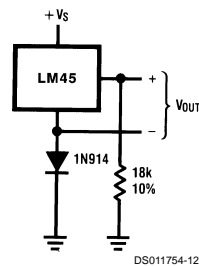
FIGURE 6. Temperature Sensor, Single Supply, -20^{\circ}\text{C} to +100^{\circ}\text{C}
