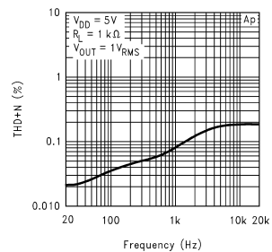
THD+N vs Frequency, 1 kΩ
