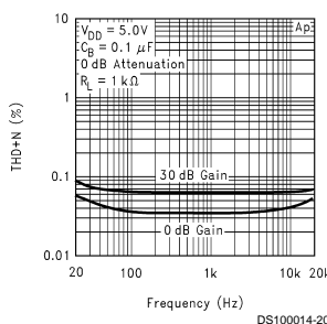
Mic Amplifier THD+N vs Frequency
