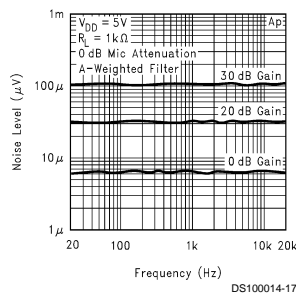
Mic Amplifier Noise Floor
