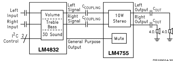
10W/ch System with I 2 C Controlled Tone, Volume and 3D Sound
