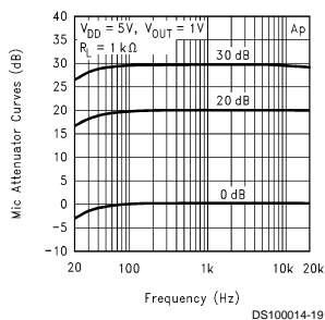
Mic Amplifier Gain vs Frequency
