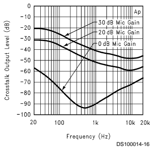
Mic Amplifier Crosstalk from Power Amplifier
