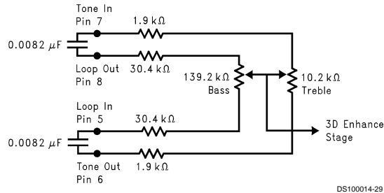
FIGURE 6. Tone Control Diagram
