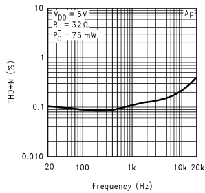
THD+N vs Frequency, 32Ω
