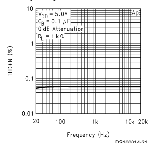
Loop-out THD+N vs Frequency
