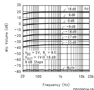
Mic Amplifier Attenuation vs Frequency
