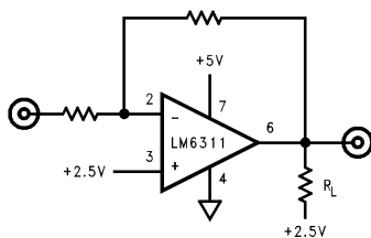
Center-referenced Output
