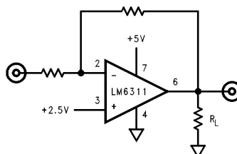
Ground-referenced Output
