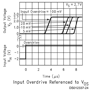
Response Time for Various Input Overdrives -t_{PLH}
