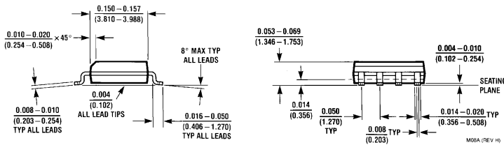
8-Pin Small Outline Package Order Number LMC7211AIM, LMC7211BIM, LMC7211AIMX or LMC7211BIMX NS Package Number M08A
