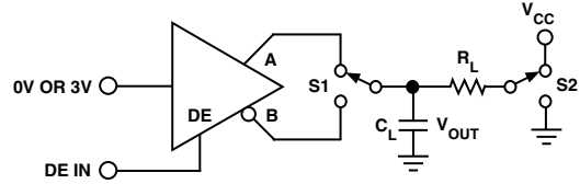
Figure 4. Driver Enable/Disable Test Circuit
