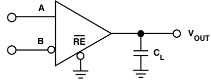
Figure 5. Receiver Propagation Delay Test Circuit
