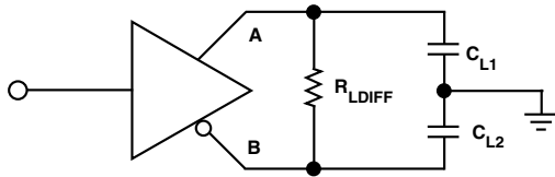
Figure 3. Driver Propagation Delay Test Circuit
