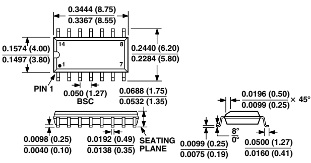
14-Lead Narrow Body (SOIC) (R-14)
