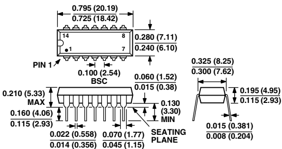
14-Lead Plastic DIP (N-14)
