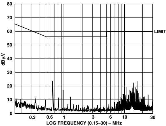
Figure 15. Conducted Emissions
