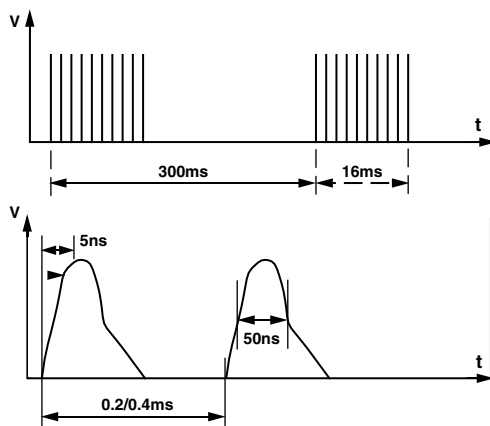
Figure 11. IEC1000-4-4 Fast Transient Waveform
