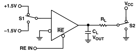
Figure 4. Receiver Enable/Disable Test Circuit
