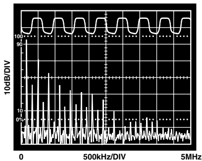
TPC 7. Driver Output Waveform and FFT Plot Transmitting @ 150 kHz
