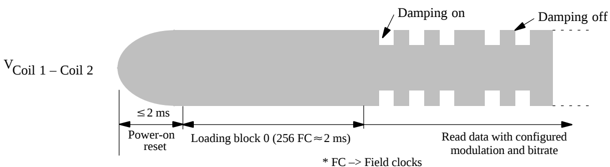
Figure 9. Voltage at Coil1/Coil2 after power-on
