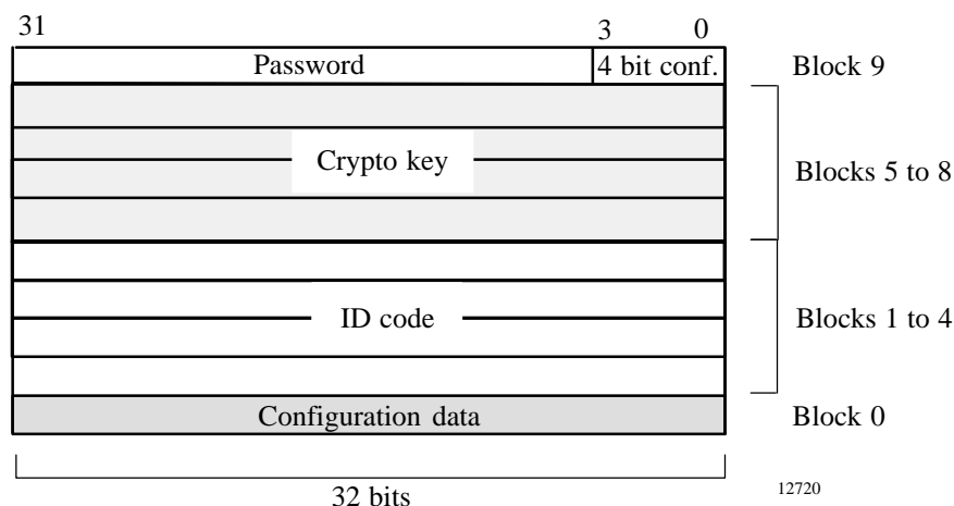
Figure 5. Memory map
