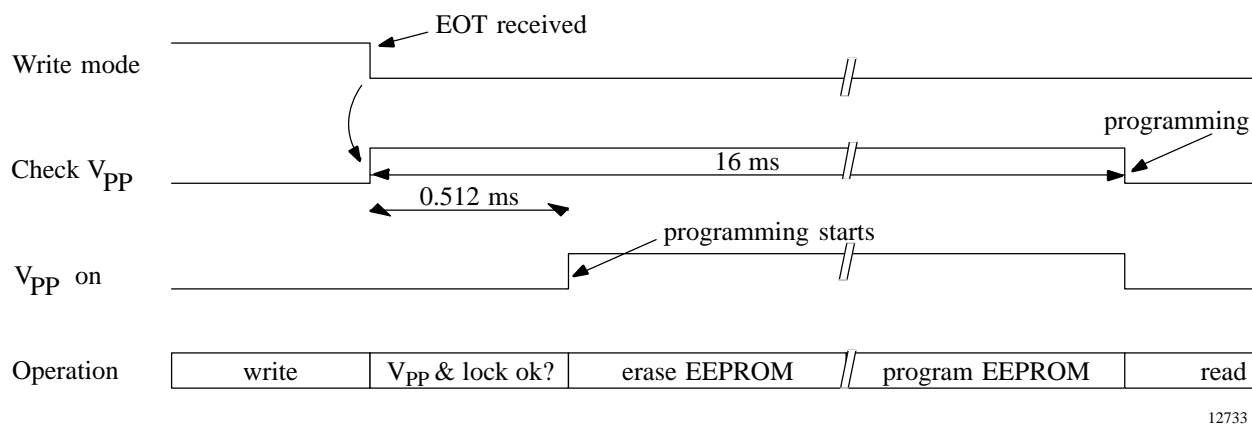
Figure 18. Programming
