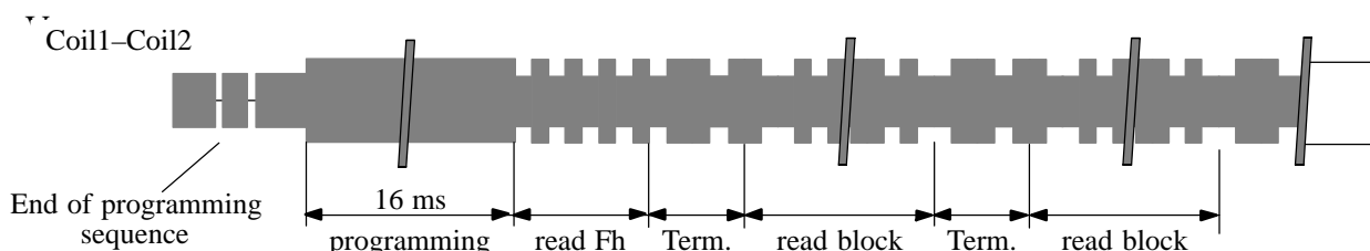
Figure 19. Programming mode datastream
