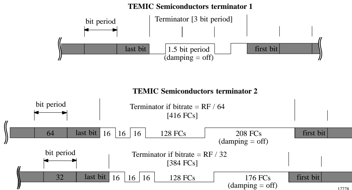
Figure 13. Terminators
