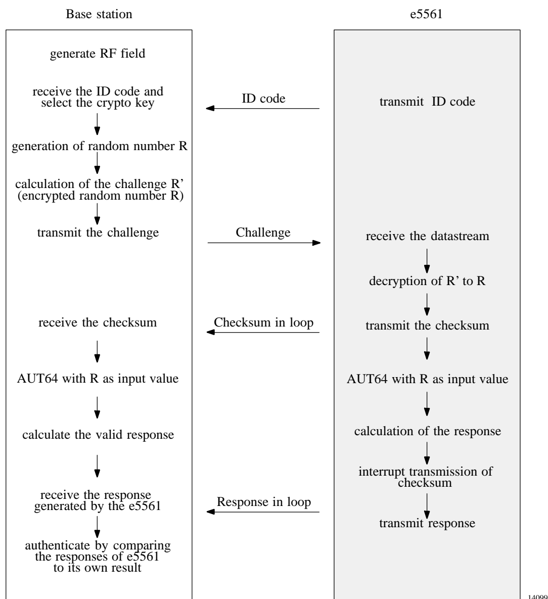
Figure 32. Authentication procedure
