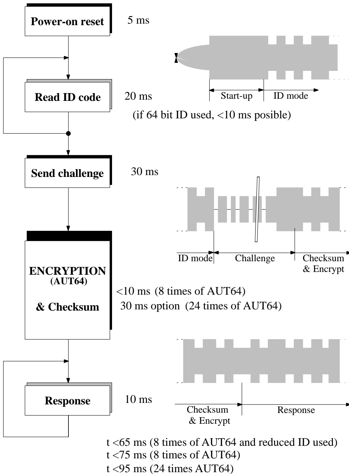
Figure 34. Authentication example
