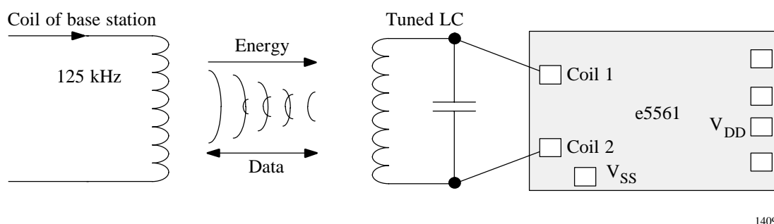
Figure 6. Application circuit
