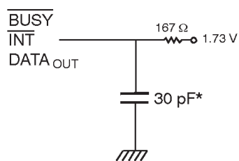
Figure 2. Output Load.
