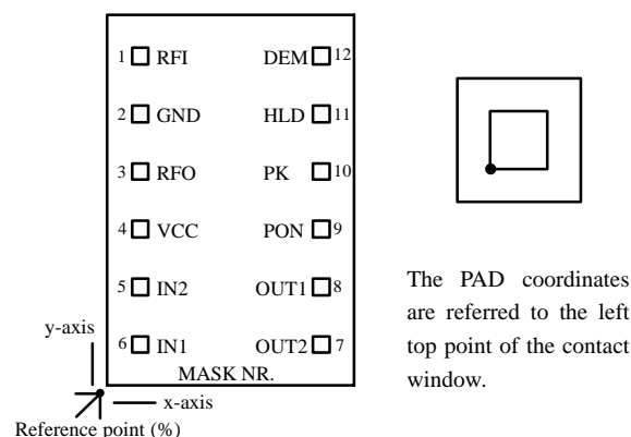
Figure 2. Pad layout
