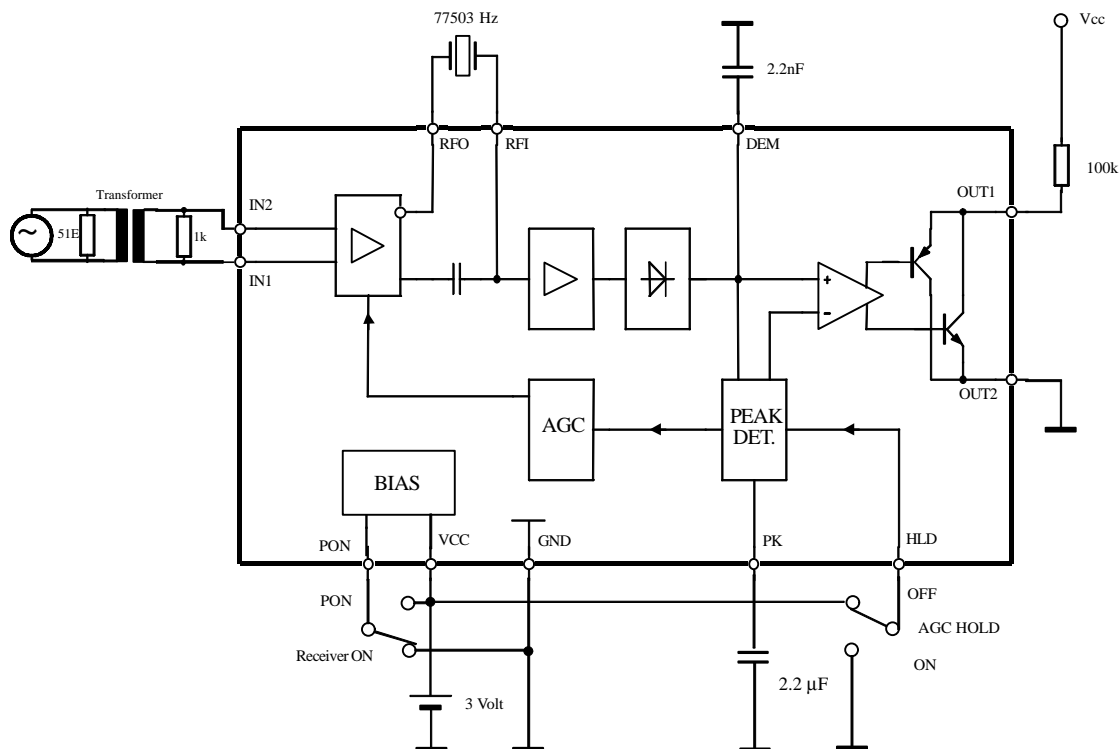
Figure 13. Test circuit
