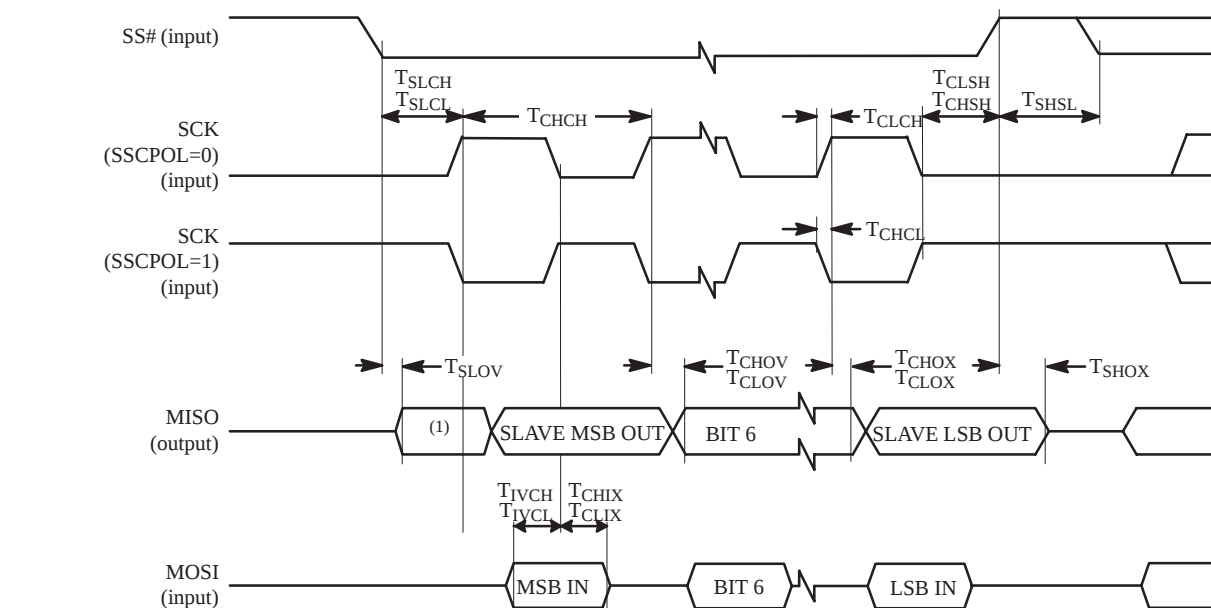
Figure 29. SPI Slave Waveforms (SSCPHA= 1)
