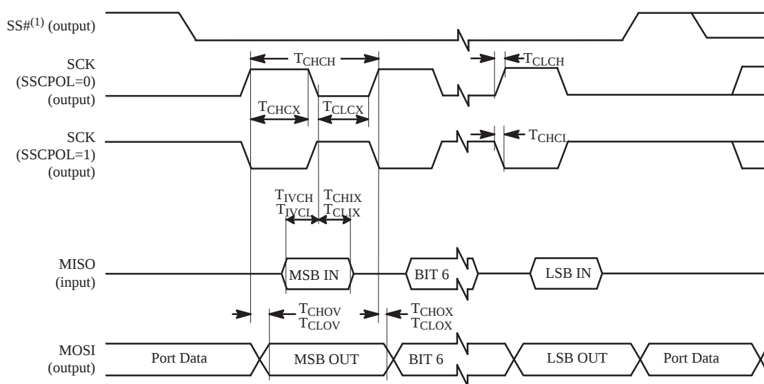
Figure 27. SPI Master Waveforms (SSCPHA= 1)
