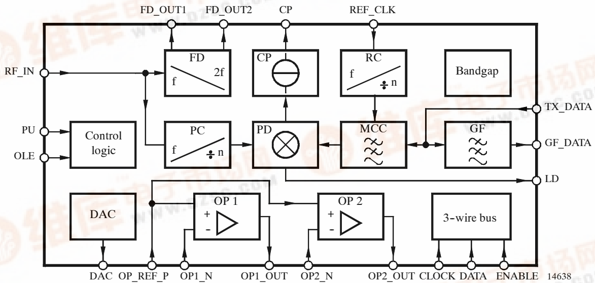
Figure 1. Block diagram
