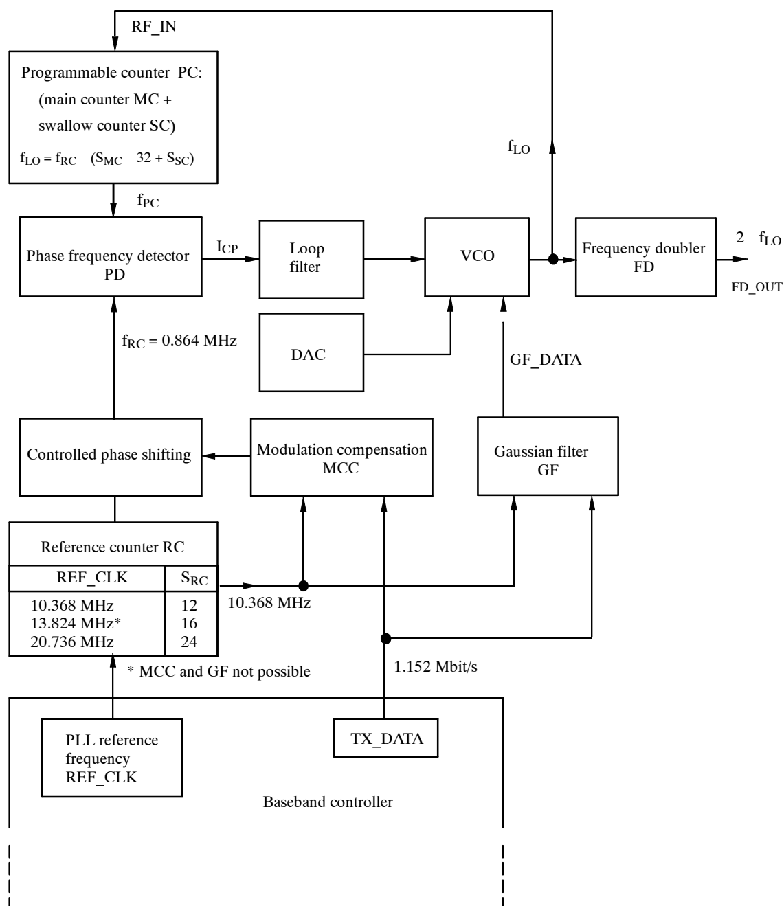
Figure 3. PLL principle
