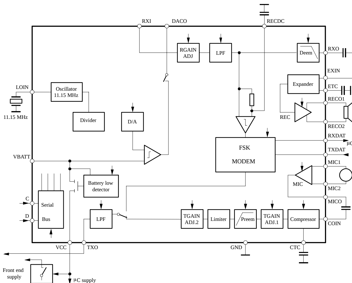
Figure 12. Application circuit
