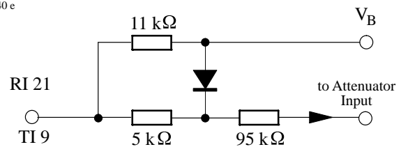
Figure 3. Attenuator input stage
