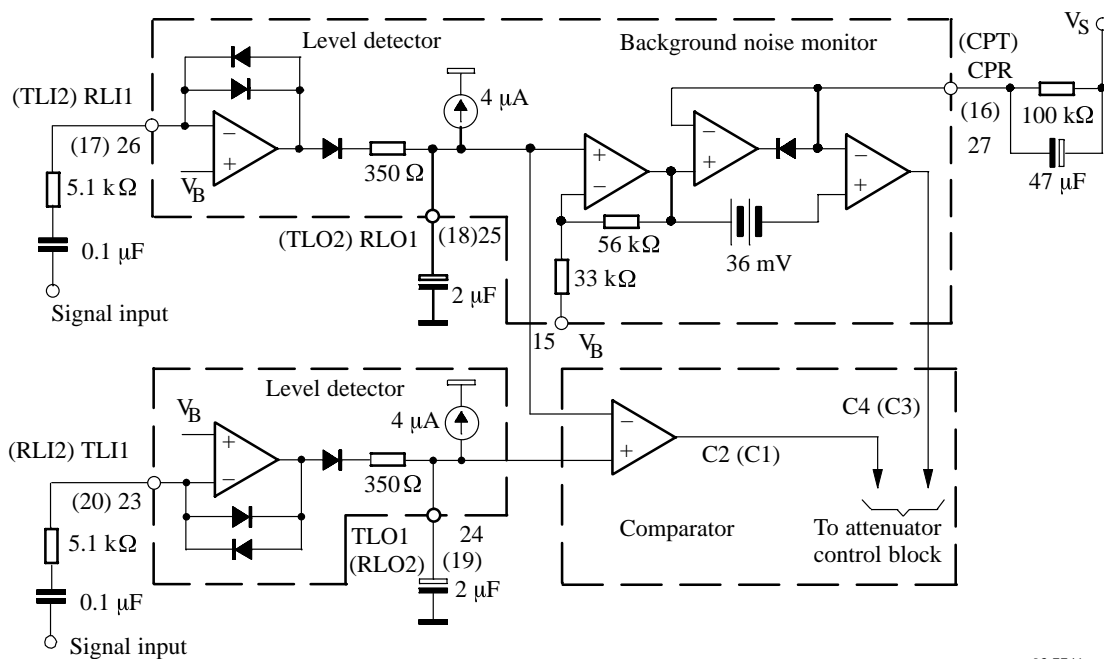
Figure 4. Level detectors
