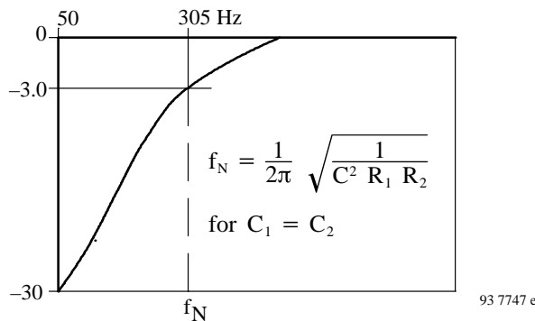
Figure 8. High-pass filter
