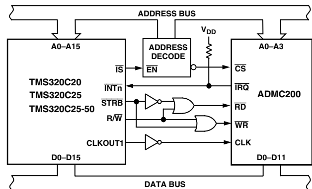
Figure 12. TI Second-Generation Devices TMS320C20/ C25/C25-50
