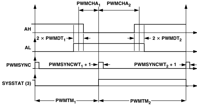
Figure 13. Typical PWM Outputs of Three-Phase Timing Unit in Double Update Mode (Active LO Waveforms)
