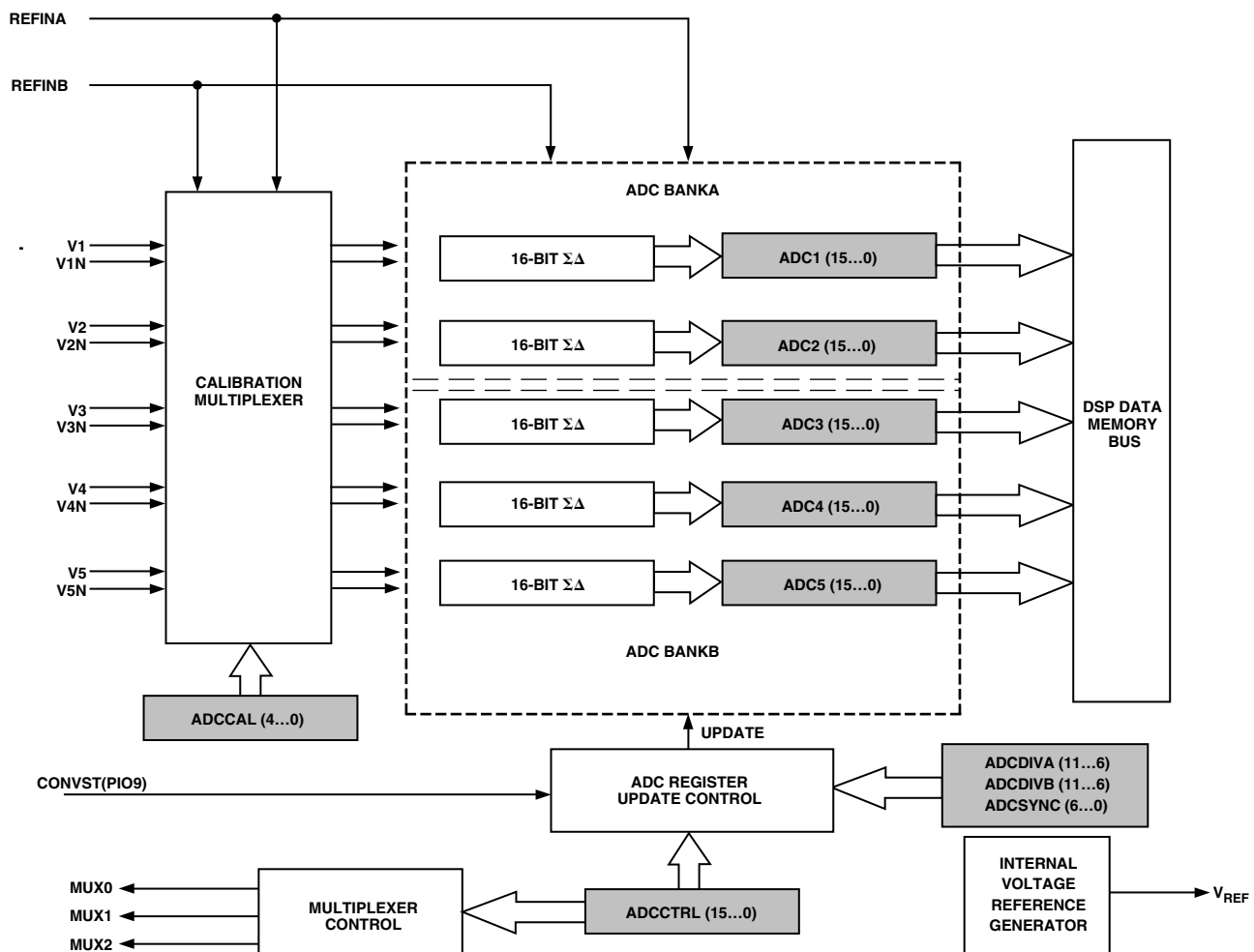
Figure 5. Functional Block Diagram of ADC System of ADCM300
