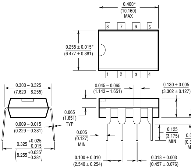
N8 Package 8-Lead PDIP (Narrow 0.300) (LTC DWG # 05-08-1510)
