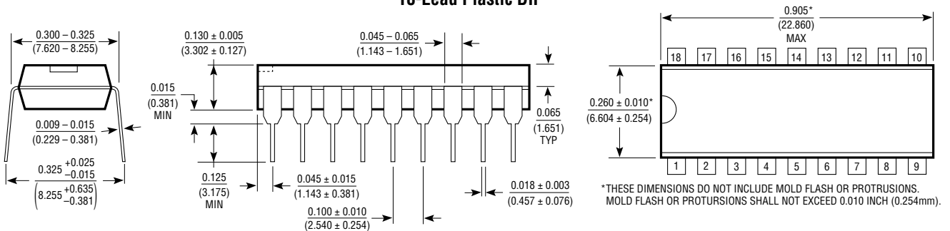
N Package 18-Lead Plastic DIP
