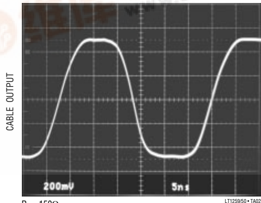
Square Wave Response
