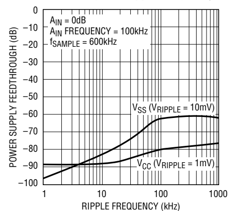
Bipolar Mode Power Supply Feedthrough vs Ripple Frequency
