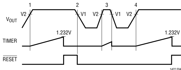
Figure 4. Supply Monitor Waveforms
