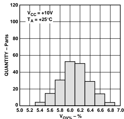
Figure 18. Overtolerance Comparator Distribution ( V_{OV\%} )
