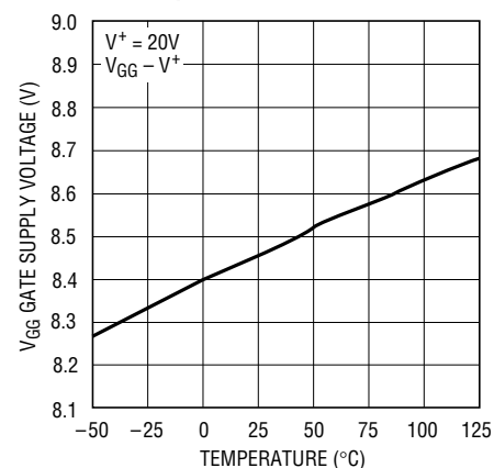
V_{\text{GG}} Gate Supply Voltage vs Temperature
