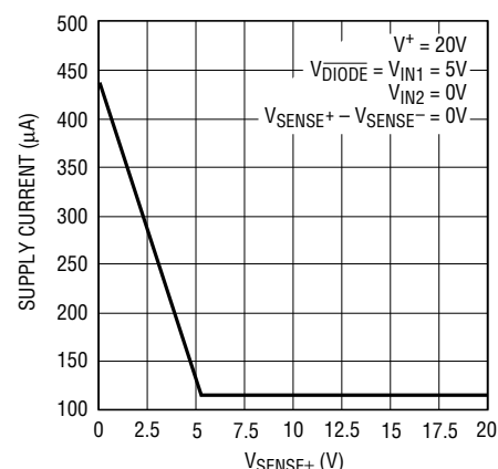
DC Supply Current vs V_{\text{SENSE}}^\pm
