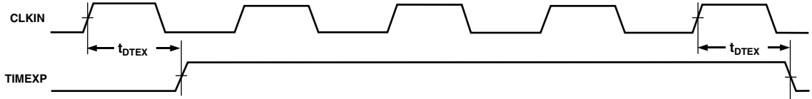
Figure 11. Timer
