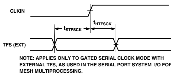
Figure 22. Serial Ports
