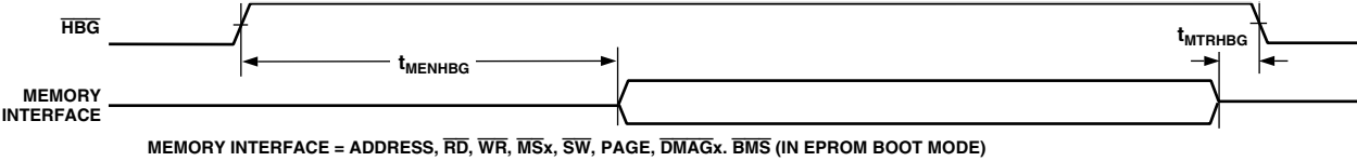
Figure 19b. Three-State Timing (Host Transition Cycle)
