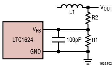
Figure 2. Setting the LTC1624 Output Voltage
