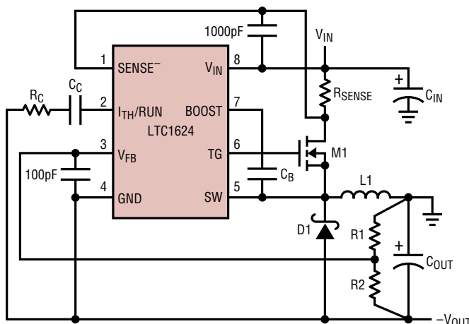
Figure 8. Positive-to-Negative Converter
