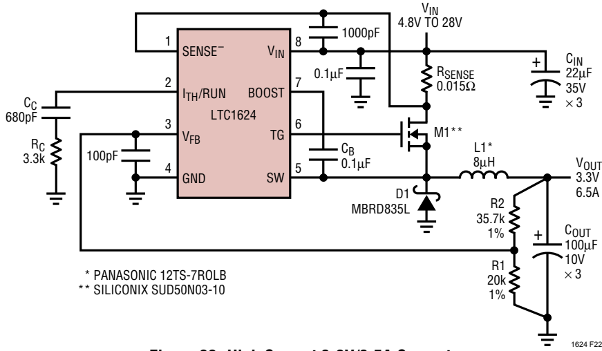
Figure 22. High Current 3.3V/6.5A Converter
