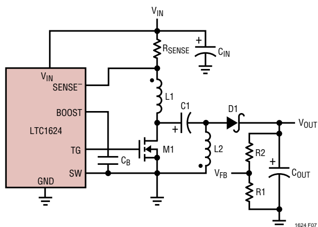
Figure 7. SEPIC Converter
