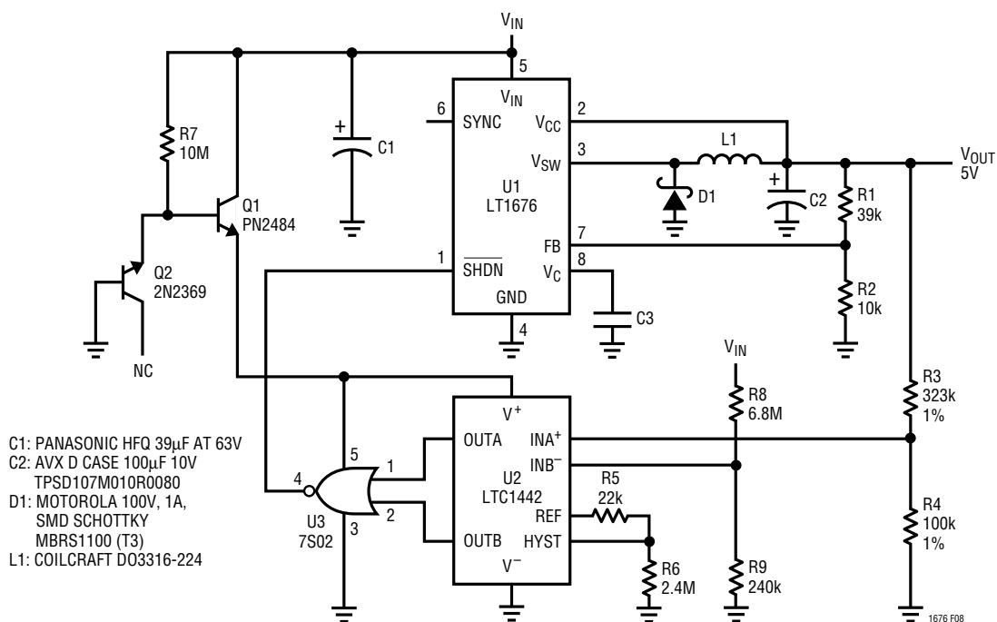
Figure 8. Burst Mode Operation Configuration with Micropower UVLO
