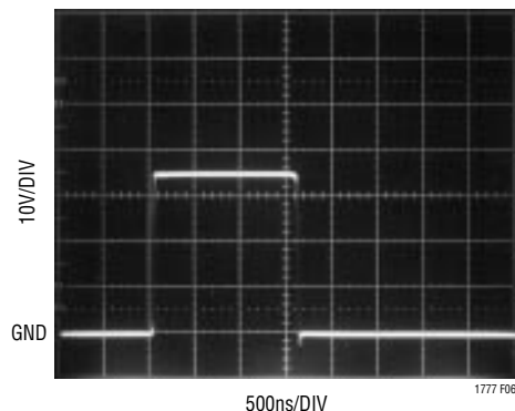
Figure 6. LT1676 V_{SW} Node Voltage Behavior for Comparison Purposes Only, V_{IN} = 36V
