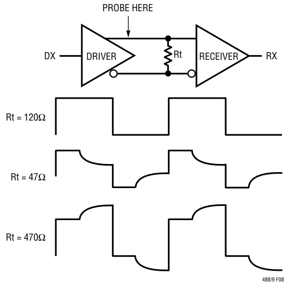
Figure 8. Termination Effects
