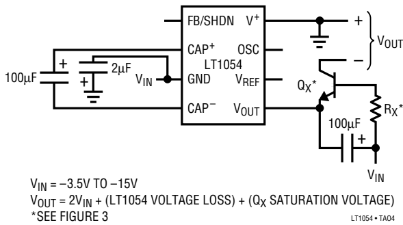
Negative Voltage Doubler
