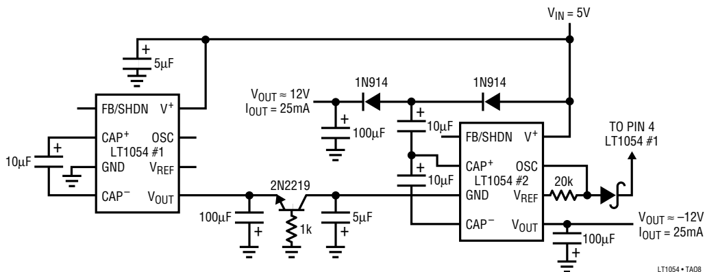
5V to \pm 12V Converter
