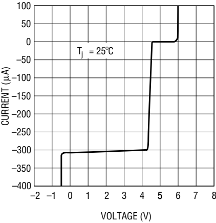
I LIM Pin Characteristics
