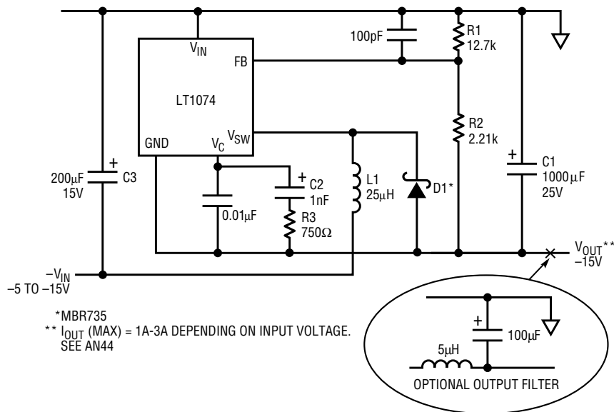
Negative Boost Converter
