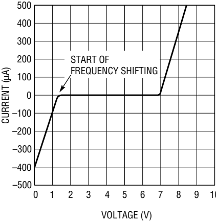
Feedback Pin Characteristics
