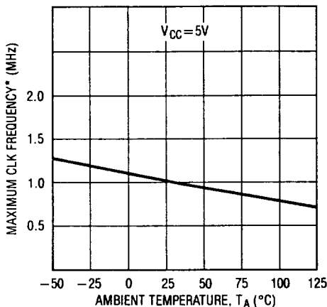
Maximum Clock Rate vs Temperature
