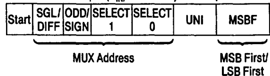
LTC1093/4 Data Input ( D_{IN} ) Word:
