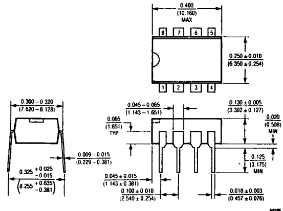
N Package 8 Lead Plastic DIP
