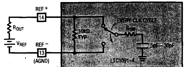
Figure 12. Reference Input Equivalent Circuit
