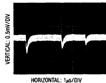
Figure 13. Adequate Reference Settling
