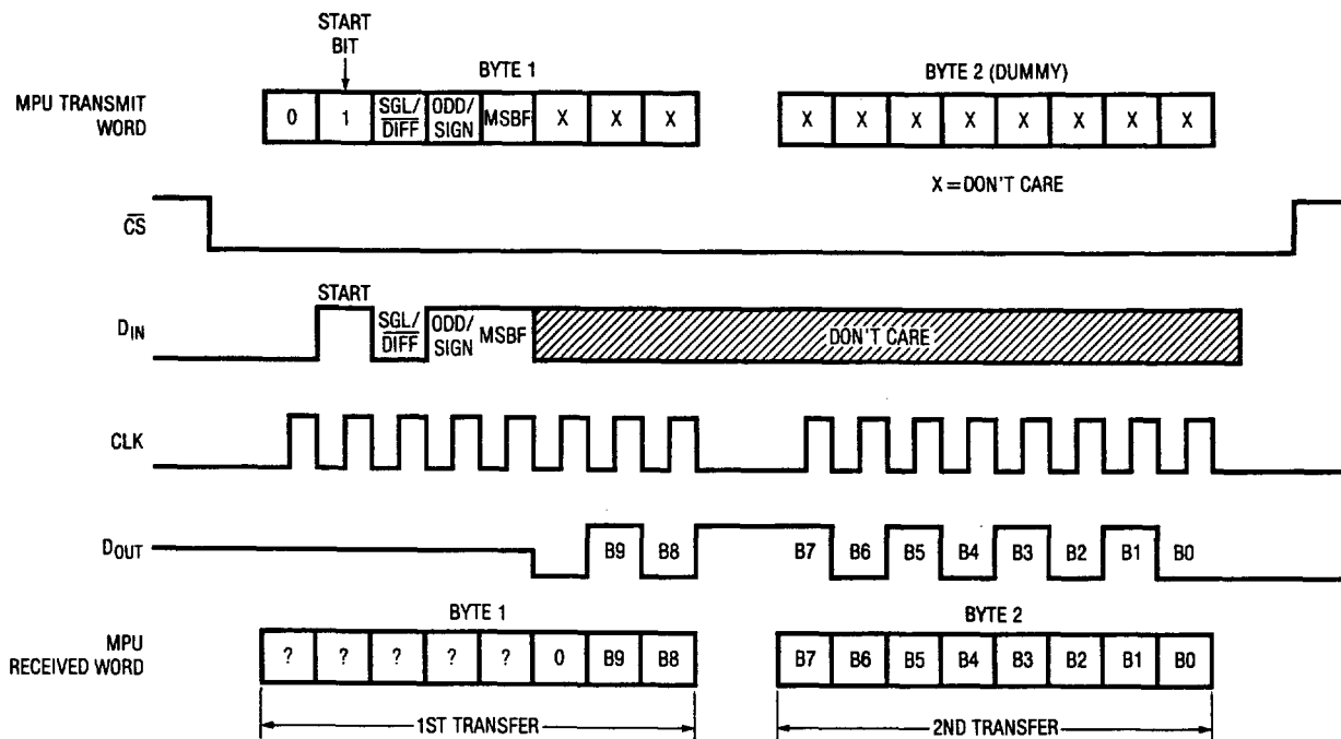
Data Exchange Between LTC1091 and MC68HC05C4
