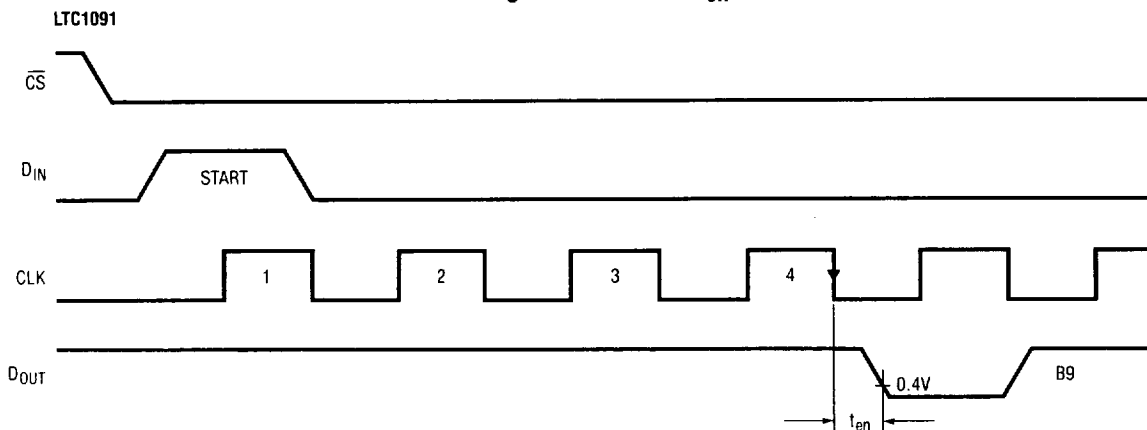
Voltage Waveforms for t_{en}
