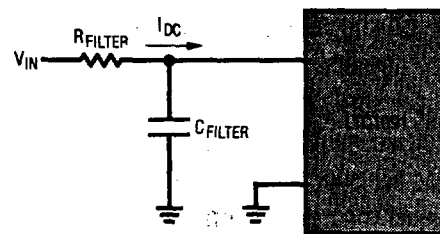
Figure 11. RC Input Filtering
